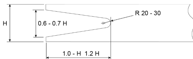
Figure 19: Typical frog-mouth tapering
