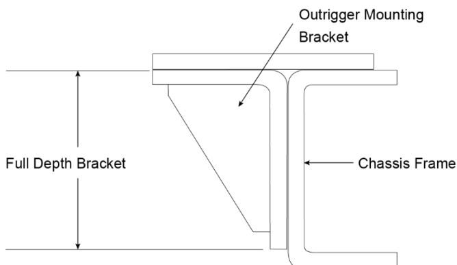
Figure 11: Details of a typical chassis mounting bracket
