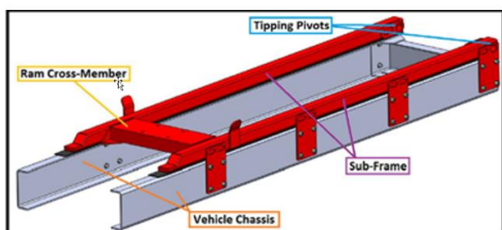
Figure 21- Basic Tipper Sub-Frame
