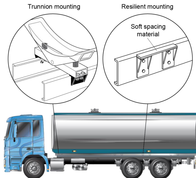
Figure 8: Typical example of tanker mounting
