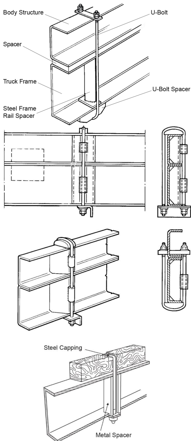
Figure 5: Typical U-bolt body mountings
