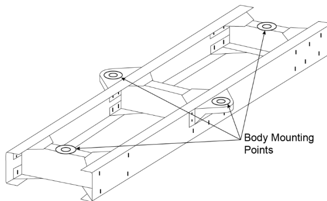
Figure 13: Typical four-point mounting
