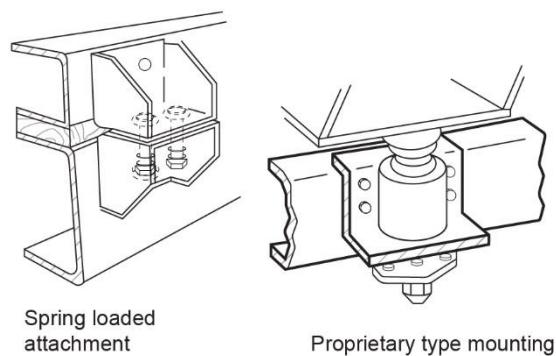
Figure 14: Typical resilient mountings
