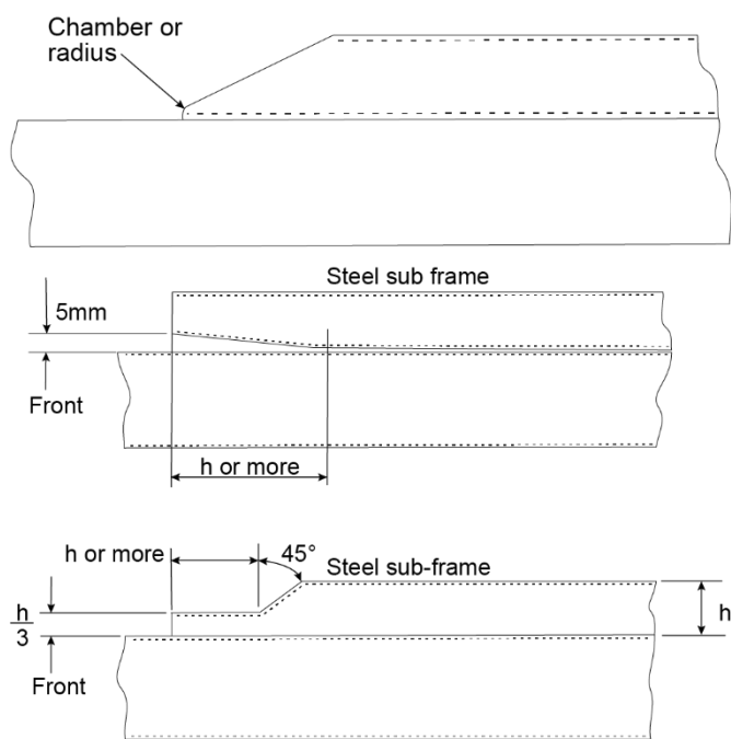
Figure 18: Examples of progressive load bearing transition
