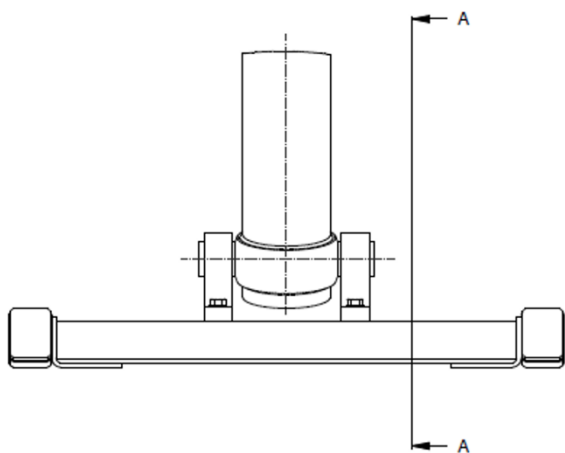
Figure 25 - Typical installation of the hoist cylinder.
