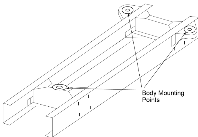
Figure 12: Typical three-point mounting
