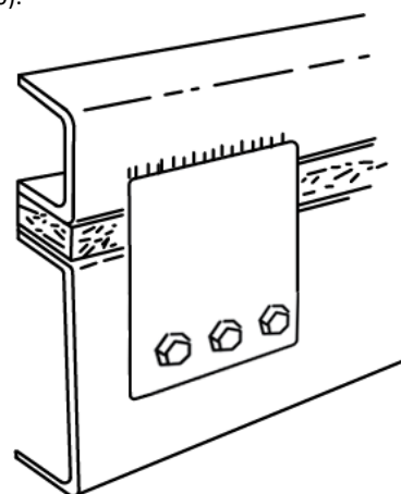
Figure 20: Typical fish plate attachment
