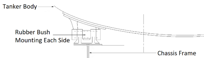
Figure 10: Details of a typical rear mounting bracket
