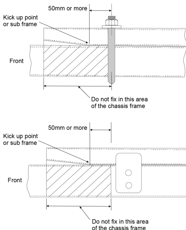
Figure 3: Attachment front end of sub-frame
