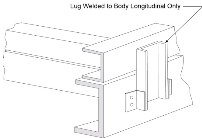
Figure 15: Additional horizontal restraint used with some body mountings
