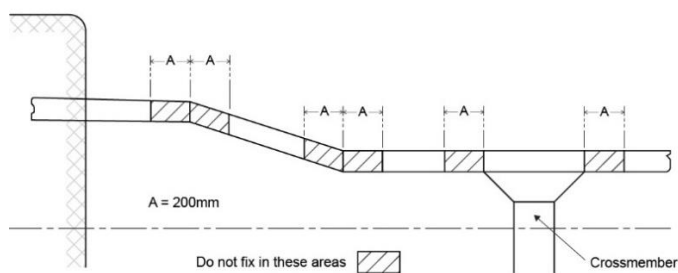
Figure 4: Attachment locations chassis
