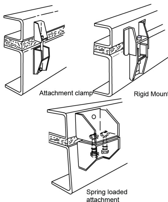
Figure 6: Typical body mounting outrigger brackets, specific to outrigger type mounts
