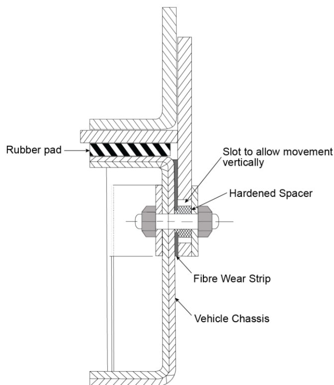
Figure 16: Body mounting with vertical compliance and friction clamping
