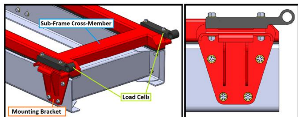
Figure 26 - Option 1 Example: Load cells w/ integrated pivot mounted on brackets & integrated into sub-frame
