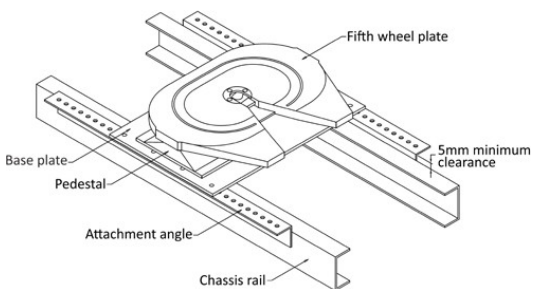
Figure 3.1 Fixed base fifth wheel assembly
