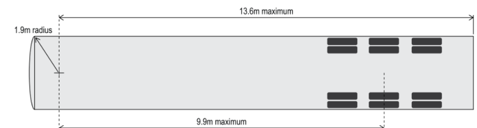
Figure 16.2 Refrigerated semitrailer
