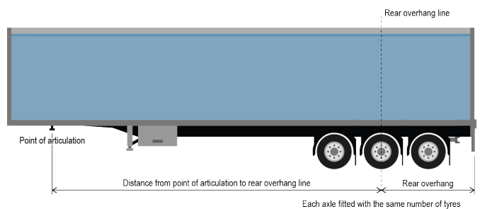
Figure 16.6 Semitrailer
