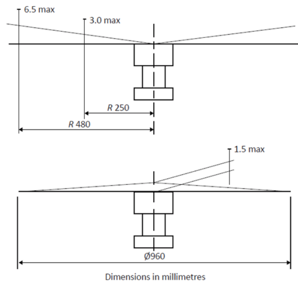
Figure 14.2 Skid plate flatness limits
