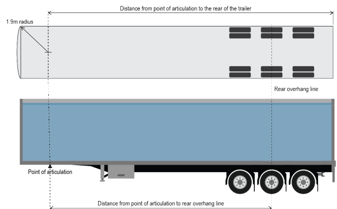
Figure 16.1 Semitrailer
