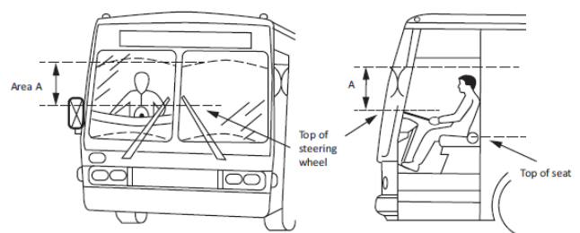
Figure 10.1 Driver's field of vision
