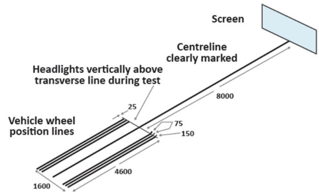
Figure 8.2 General arrangement of the headlight testing space
