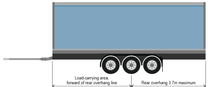
Figure 16.5 Pig trailer
