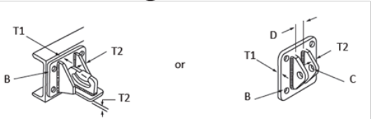
Figure 3.6 Typical attachment of chains
