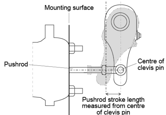
Figure 2.2 Measuring stroke length
