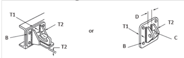
Figure 14.5 Typical attachment of chains
