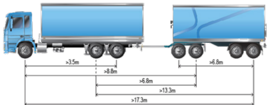
Figure 2 - Truck and four axle dog trailer minimum axle spacing
